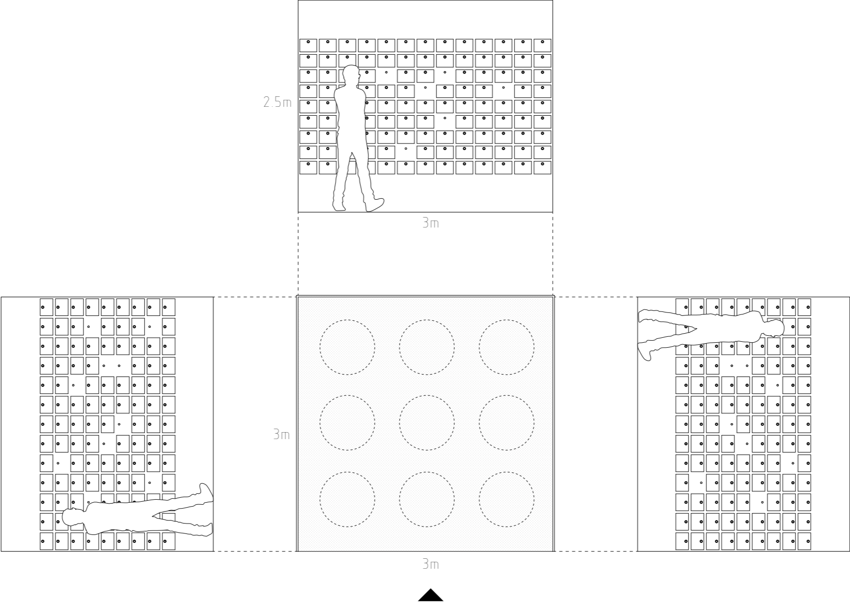
3/4 PLAN & ELEVATIONS
